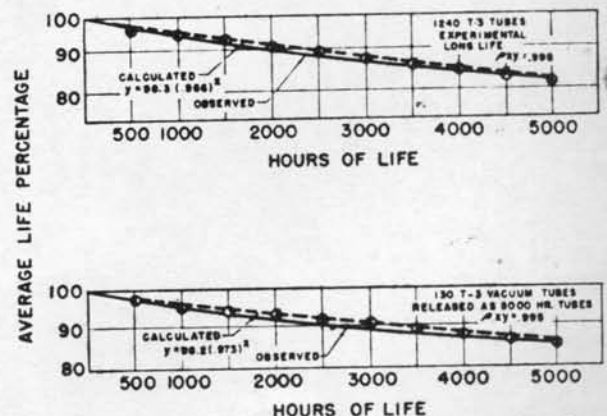
Fig. 1—Life survival curves: y = ab^x . Observed data and calculated curves for two heterogeneous groups of longer-life tubes.
